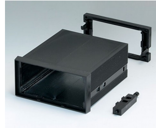
B6032031 DIN-MODULAR CASE TYPE A, Vers. I PPO (UL 94 V-0) black RAL 9005 96x48x100mm
